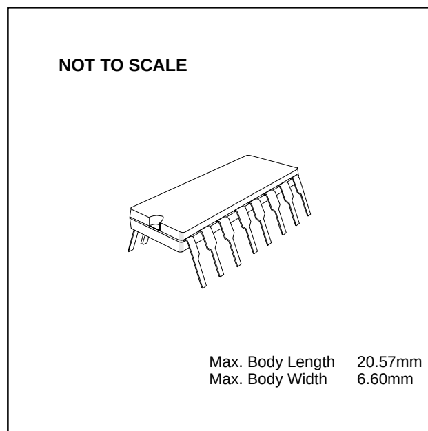
FX128P3 16-pin Plastic DIL (P)
